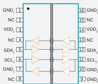
Figure 2. NSI8200-DSWR Block Diagram
