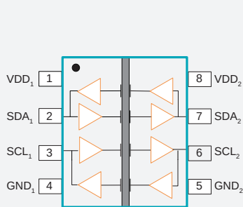
Figure 1. NSI8200-DSPR & NSI8200-DSWWAR Block Diagram
